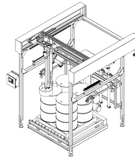
MT-55T Automatic Drum and Tote Filler
