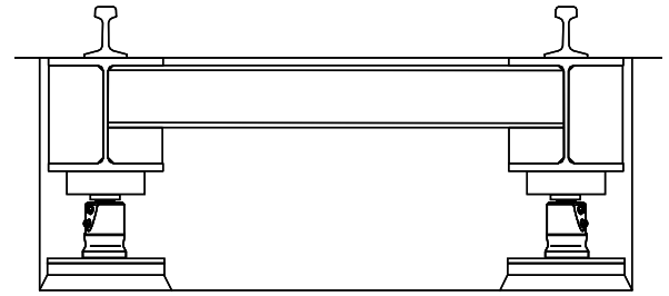
VRS241 Cross Section
